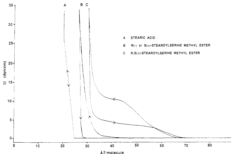
Figure 5. Surface pressure–area isotherms for the compression–expansion cycle of (A) stearic acid, (B) R (-)- or S (+)-stearoylserine methyl ester, and (C) RS (±)-stearoylserine methyl ester on a pure water subphase at 25 °C and compressed at 29.8 Å 2 /molecule/min.
